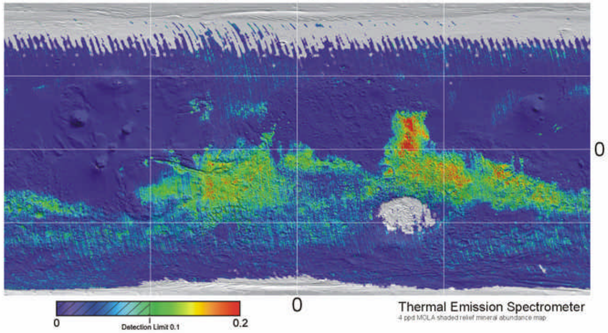
Figure 3. Concentration map of high-calcium pyroxene at 4 pixels per degree. High concentrations correspond to basaltic surfaces. Mineral concentration maps are available in digital and image formats at 1, 2 and 4 ppd.
